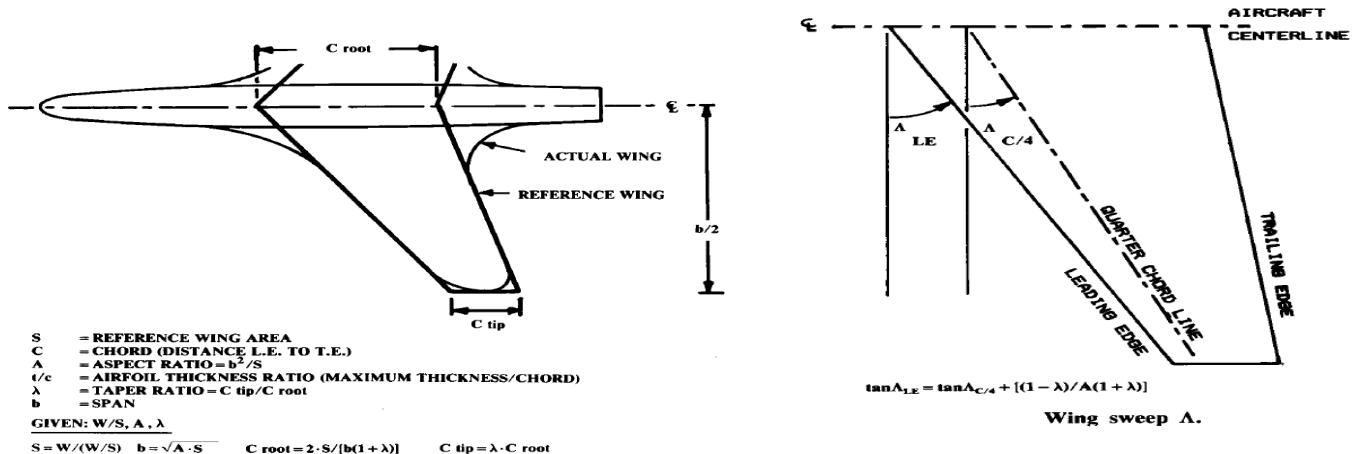
FIG 9a & 9b: Wing Design
