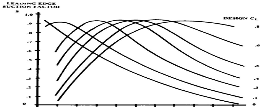
FIG 10: Grapg For Design CL
