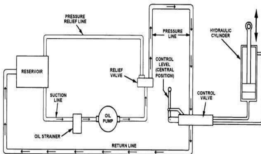
FIG: BASIC HYDRAULIC SYSTEM.
