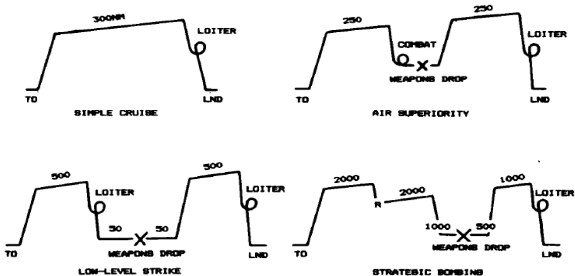
FIG 8: Mission Profiles of Various Aircrafts
